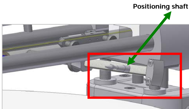
Pic. 8: Turning the headshell
