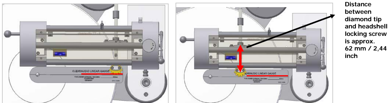
Pic.17: Adjustment of the linear tracking
