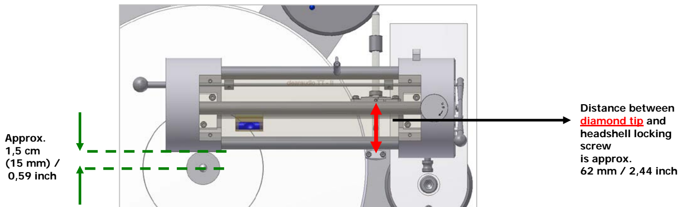
Pic. 10: Correct position of the headshell
