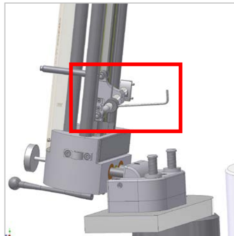
Pic.13: Locking the counterweight(s)
