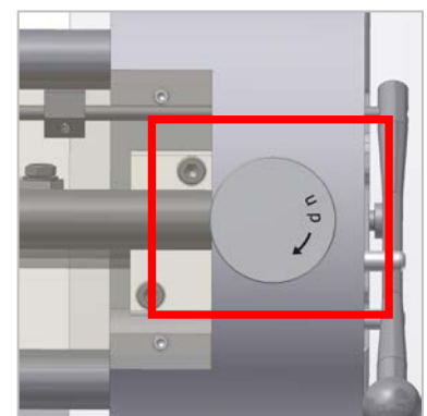
Pic.14: Height adjustment
