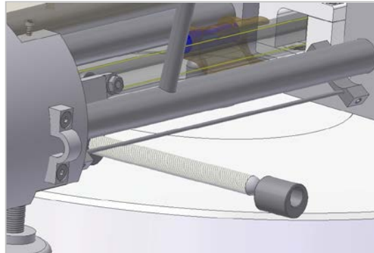
Pic.12: Set up of counterweight(s)
