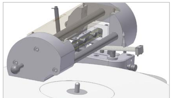
Pic. 7: Setting up the headshell
