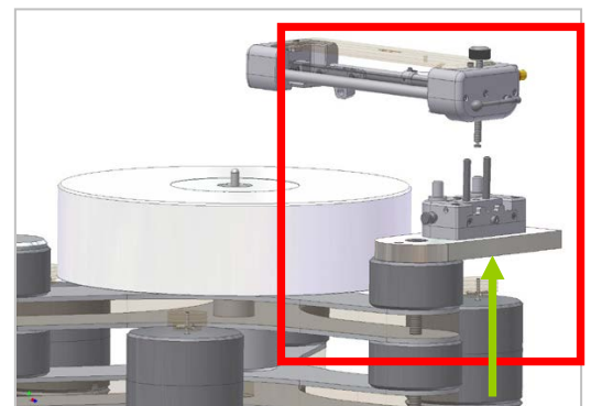
Pic.5: Placing the tonearm on the tonearm base
