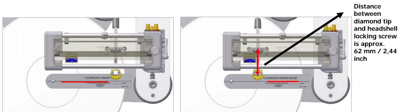
Pic.18: Adjustment of the linear tracking
