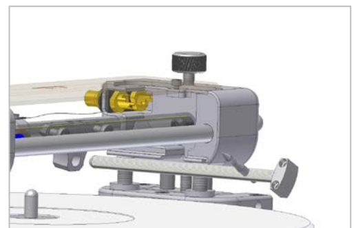
Pic.7: Setting up the headshell
